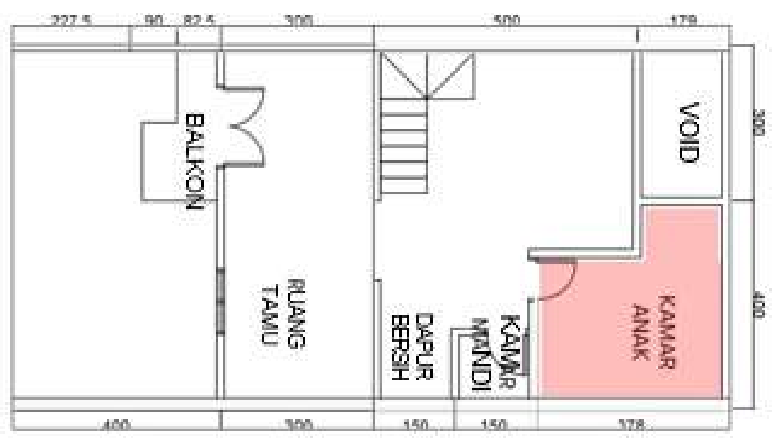
LANTAI II
